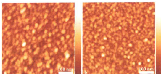
FIG. 11. (Color online) AFM images of (a) tetramer and (b) octamer fragments deposited on mica substrate. Image size is 500 \times 500 nm 2 . Z (vertical) ranges are 4.0 (a) and 4.1 (b) nm.
