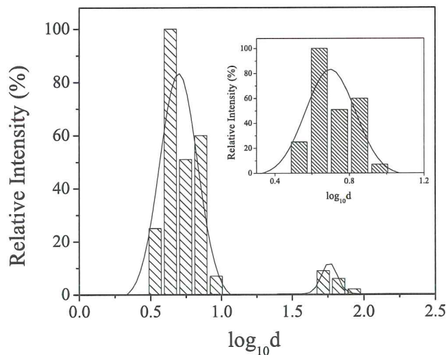
FIG. 8. Two populations, octamers and aggregates, are shown at 20 °C and 20°. In the inset the fragment population is reported.
