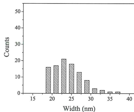
FIG. 18. Histograms of width distribution for octamers near isoelectric point.
