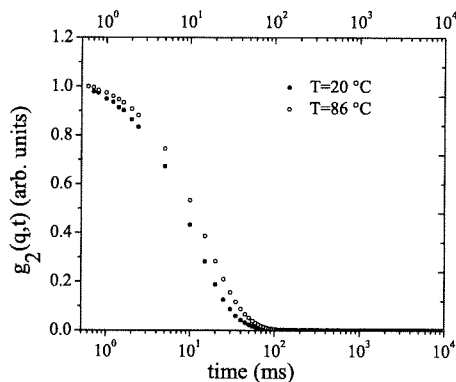
FIG. 2. DLS normalized experimental correlation functions at 90^\circ for octamer solutions.
