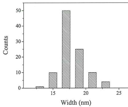
FIG. 15. Histograms of width distribution for octamers.
