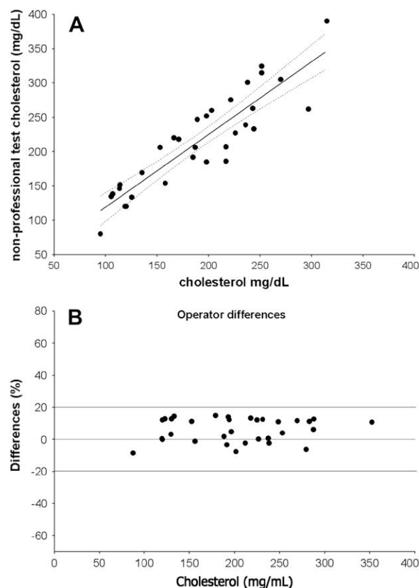
Fig 2. Passing-Bablok regression for cholesterol in practicability test ( n = 32 ) ( y = 1.1208x - 20.677 ) (A). Differences in results obtained by nonprofessionals compared with professionals (B).
