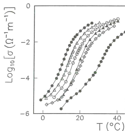
FIG. 2. \sigma(T) at W/S = 11 for the same \phi values as Fig. 1 with identical symbol meaning.
