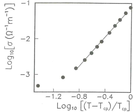
FIG. 4. Application of the scaling law to the points above threshold at \phi = 0.327 .
