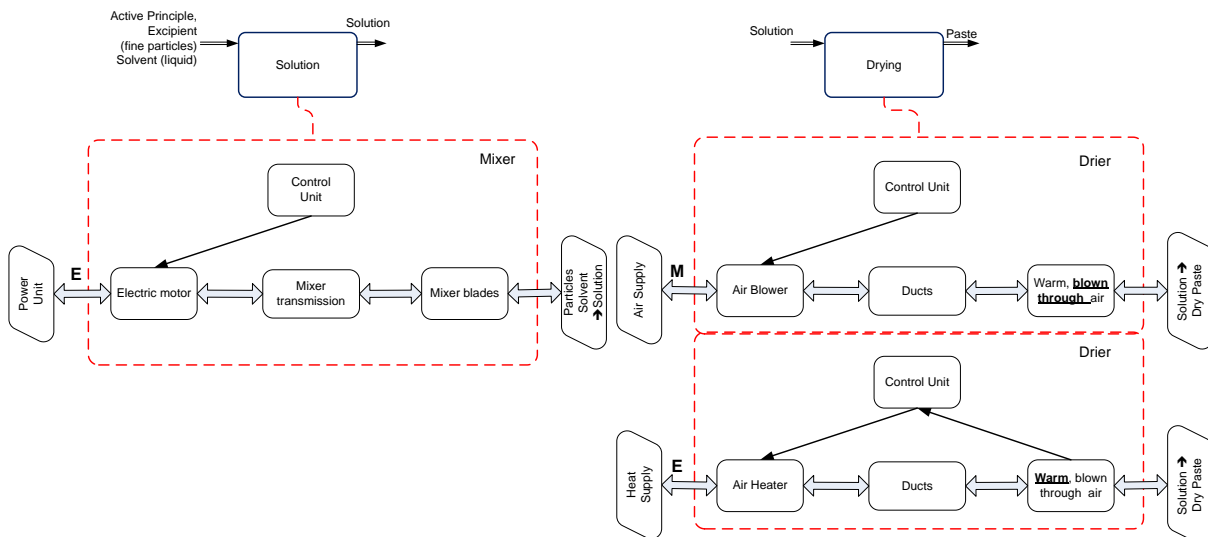
Figure 6. Exemplary Behaviors of the first two elementary functions of figure 4 represented through the TRIZ minimal model of a technical system.
