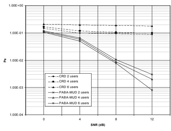
Fig. 2 Performance comparison between conventional RAKE detector (CRD) and pre-combining advanced blind adaptive multiuser detector (PABA-MUD) in the uplink GSM sub-urban channel with different number of asynchronous interfering users each one with a 10 dB stronger received power level than desired
