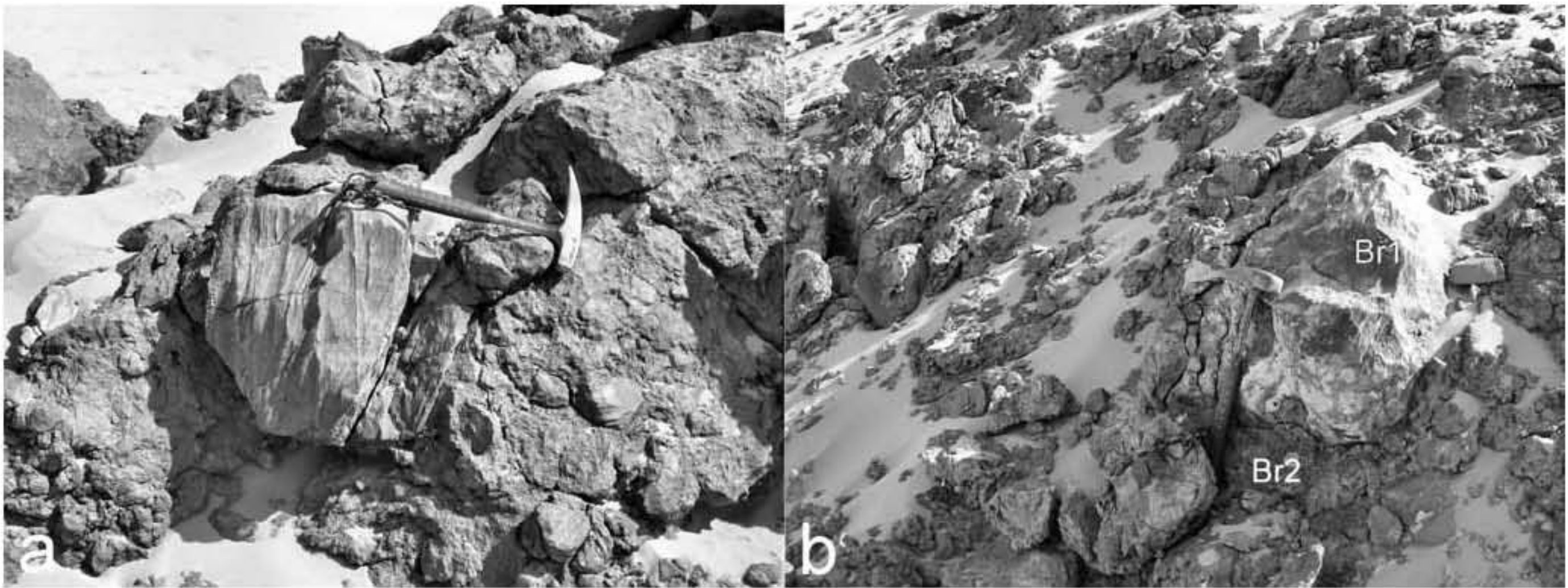
Fig. 8. Br2 breccia from GKCF1. a) Decimetric quartz-arenitic laminated boulder included in Br2 breccia. b) Br1 boulder included in Br2 breccia.
