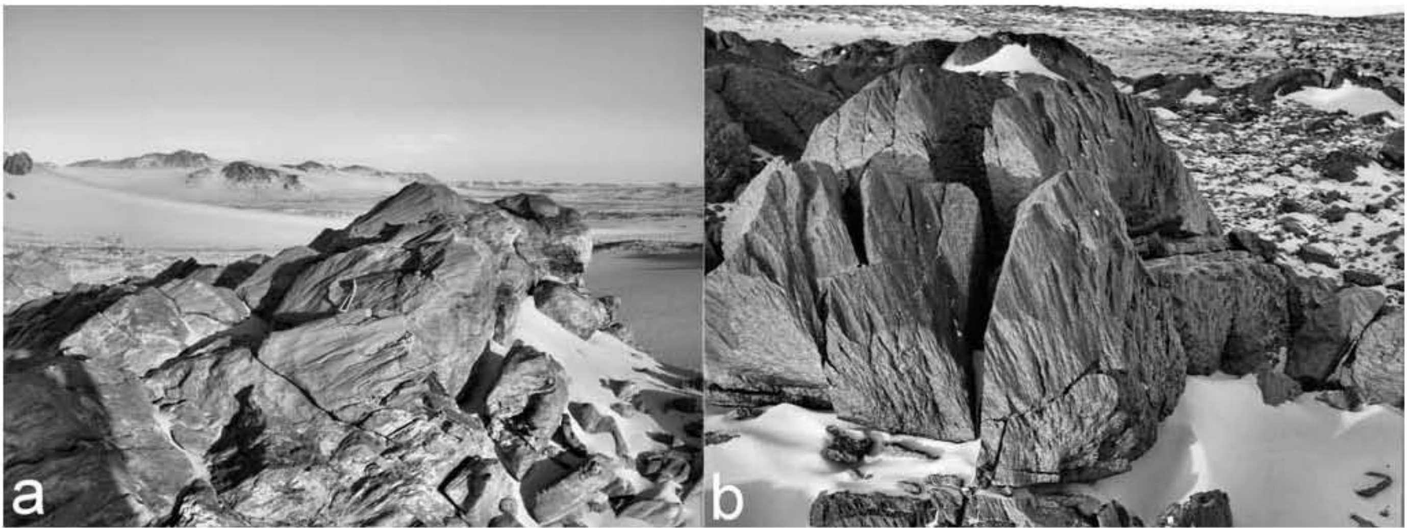
Fig. 9. Shatter cones-like features. a) Striations on quartz-arenites at GKCF13. b) Striations on basalts at El-Baz volcanic crater.
