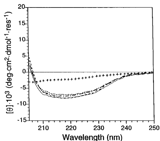
FIGURE 4: Comparison of the 205–250 nm regions of acylphosphatase CD spectra recorded in 50 mM acetate buffer, pH 3.8, at 30 °C and an enzyme concentration of 0.10–0.15 mg/mL. Wild type (—); Thr42Ala mutant (---); Thr46Ala mutant (···); Asn41Gln mutant (- - -). Thermally denatured (70 °C) wild-type enzyme is represented as (+ + +).
