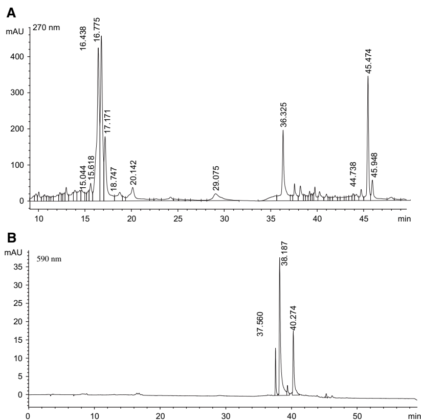
Figure 1. HPLC profiles of Hypericum perforatum L. extract. (A): HPLC profile at 270 nm. Rutin was linear from 4.5 to 100 \mu\text{g/mL} and all the curves had coefficient of linear correlation \geq .999 with y -intercepts which were close to zero. t_R = 16.43 minutes, rutin, t_R = 16.77 min., hyperoside, t_R = 17.17 minutes, isoquercitrin, t_R = 18.74 minutes, quercitrin, t_R = 29.07 minutes, quercetin, t_R = 36.32 minutes, I3, I18-biapigenin, t_R = 44.73 minutes, furohyperforin, t_R = 45.47 minutes, hyperforin, t_R = 45.94 minutes, adhyperforin. (B): HPLC profile at 590 nm. t_R = 38.18 minutes, pseudohypericin, t_R = 40.27 minutes, hypericin.
