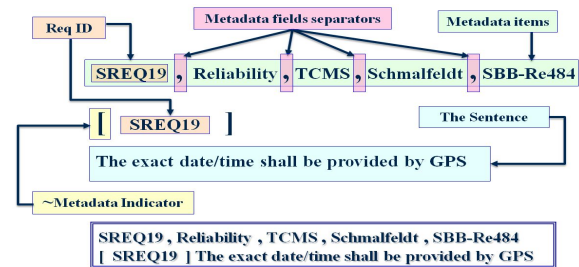
Figure 2: QUARS EXPRESS exchange data format example
