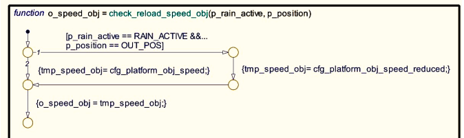
Figure 6: Example of unit requirement formalization
