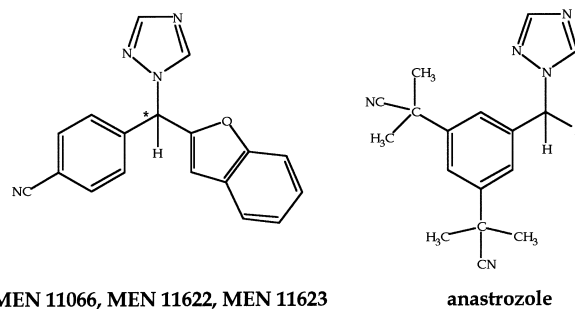
Fig. 1. Chemical structures of MEN 11066, (–)-MEN 11622, (+)-MEN 11623 and anastrozole.
