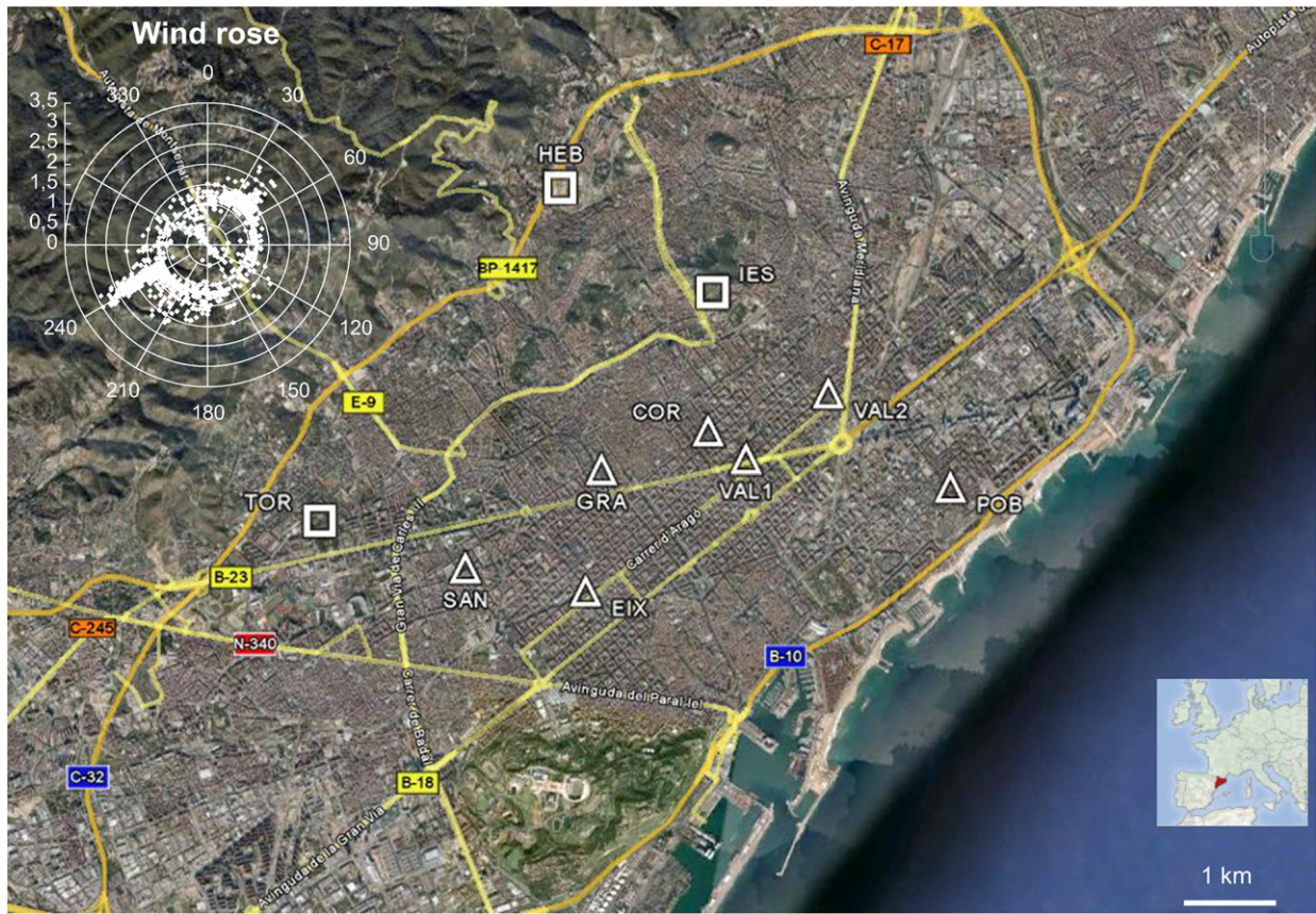
Fig. 1. Study area (main traffic routes are highlighted), location of VAL1, VAL2 and COR laboratory vans, seven reference air quality stations and wind speed (m/s) and direction. Triangles indicate traffic sites, squares indicate urban background sites.
