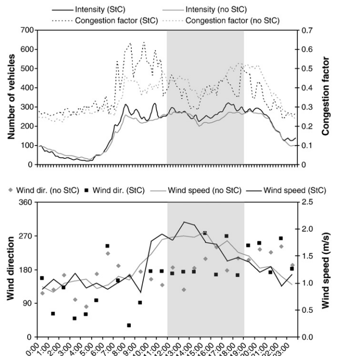
Fig. 5. Average daily evolution of traffic intensity and congestion [occupancy (%)/intensity(#)] (top) and wind speed and direction (bottom) during StC and no-StC days.
