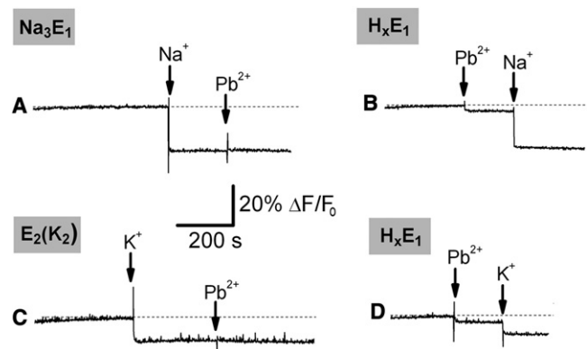
FIGURE 1 Addition of 10 \mu\text{M} \text{Pb}^{2+} to the ion-bound conformations \text{Na}_3\text{E}_1 (trace A ), \text{E}_2(\text{K}_2) ( C ), and \text{H}_x\text{E}_1 (traces B and D ). (Shading) Preferentially adopted conformation when \text{Pb}^{2+} is added. Where indicated (arrows), sodium and potassium ions are added at final concentrations of 50 mM and 20 mM, respectively. The initial fluorescence level, relative to \text{H}_x\text{E}_1 conformation, is due to RH421 dye partitioned into protein-containing membrane fragments. (Dashed line) Zero fluorescence level taken as reference.
