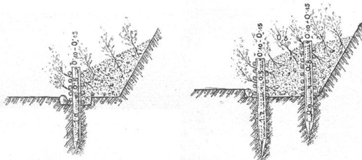
Fig. 1 – Wattles [Wang 1903]
