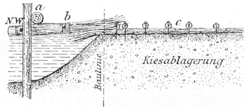
Fig. 9 – Groynes [Wang 1903]
