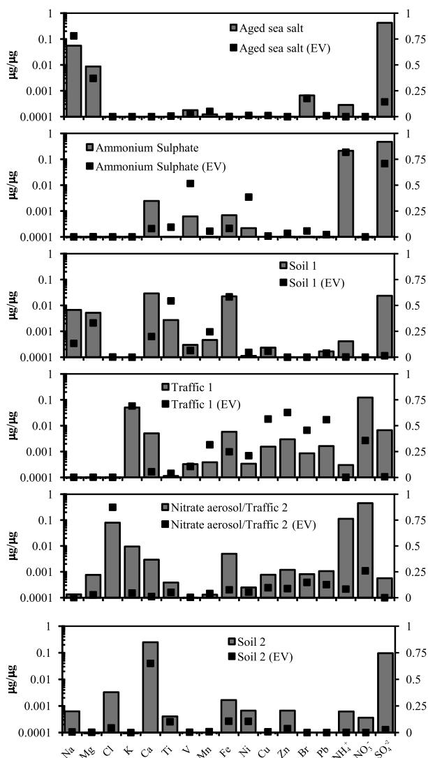
Fig. 1. Source profiles (value \pm explained variation) of the identified PM 2.5 sources measured at Elche. (Left axis: value of ion/element in the source, represented by grey bars. Right axis: explained variation, represented by dark squares).
