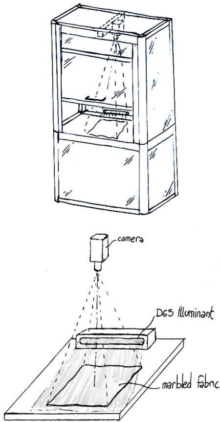
Fig. 2 MV system
