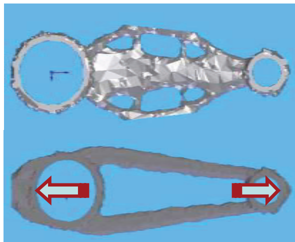
Figure 3: Optimized topologies of a connecting rod emerging from mono-goal analyses: compression (above) and traction (below) loads.
