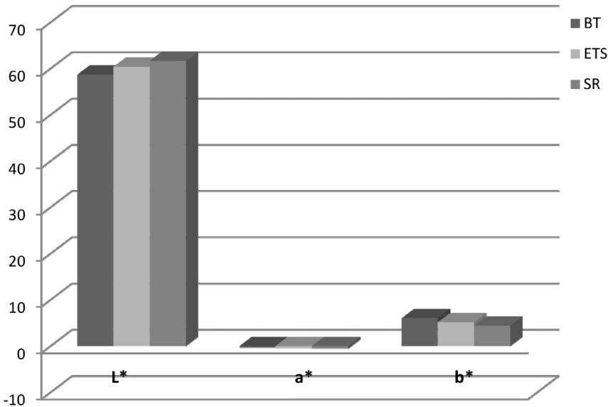
Figure 7. L*, a*, b* values of test samples before treatment and after treatment with ethyl silicates and siloxane resin.
