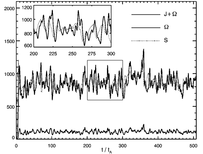
FIG. 2.—Same simulation of Fig. 1. The integrated Poynting flux S dynamically balances the ohmic ( J ) and viscous ( \Omega ) dissipation. Inset shows a magnification of total dissipation and S for 200 \leq t/\tau_A \leq 300 .
