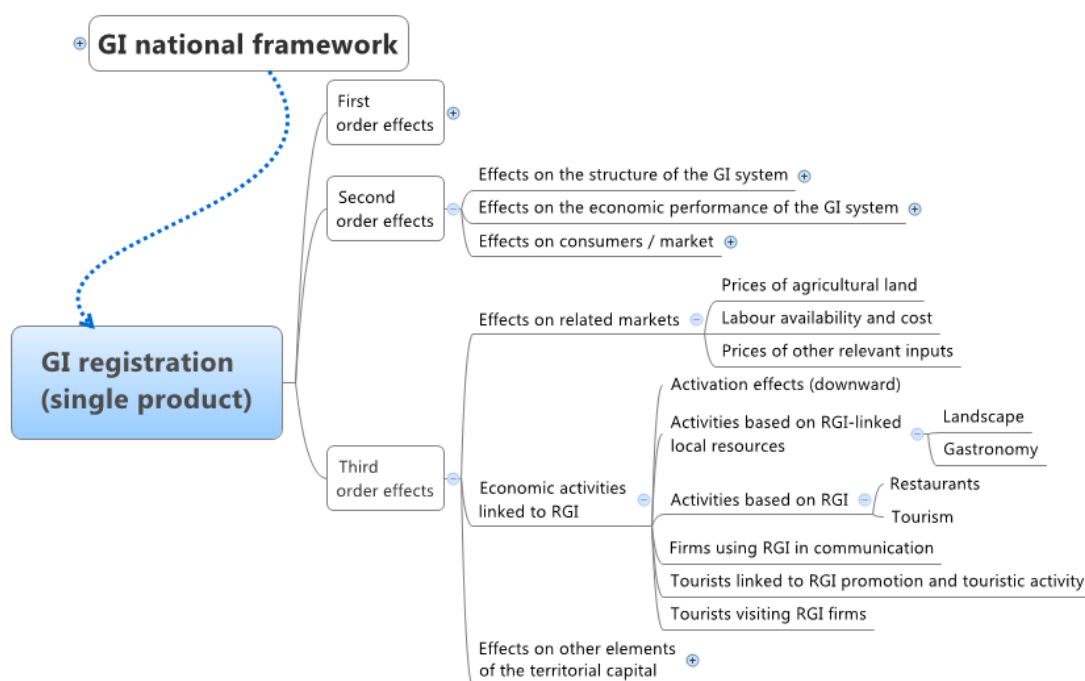
Scheme 5.6 RGI potential effects outside the GI production system
