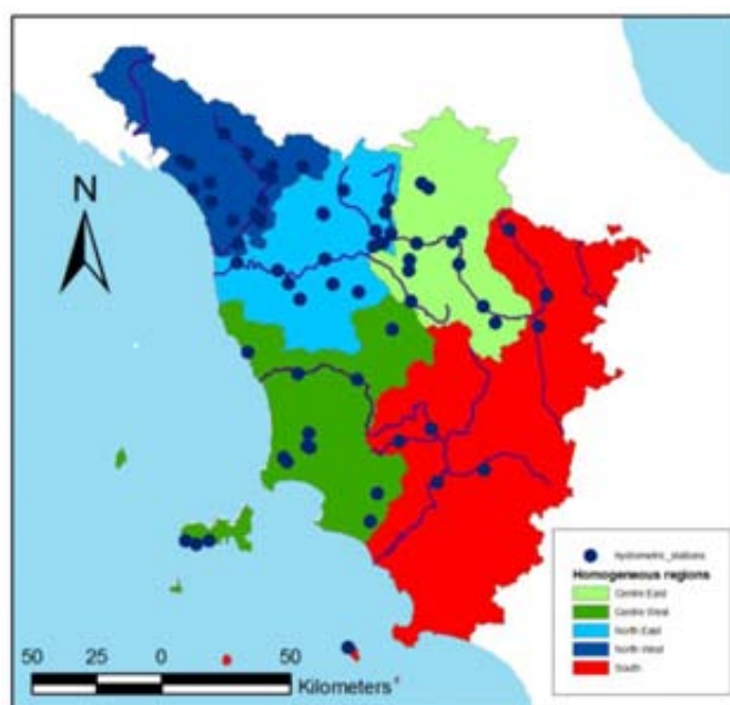
Figure 2 Subdivision in hydrologically and statistically homogenous regions.
