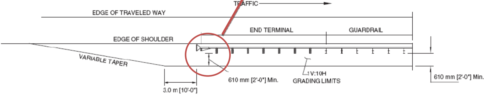
ALTERNATIVE GRADING
