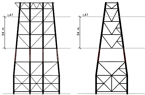
Figure 2. SASP demolition phase: vertical bracing cut
