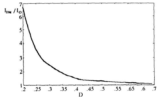
Fig. 5. Normalized maximum current I_{DM}/I_o as a function of duty cycle D .
