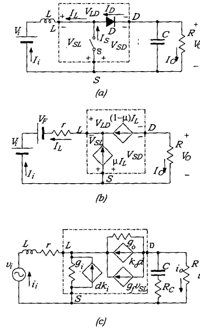
Fig. 4. PWM boost converter. (a) Schematic circuit. (b) Equivalent linearized DC circuit. (c) Equivalent linearized ac circuit.
