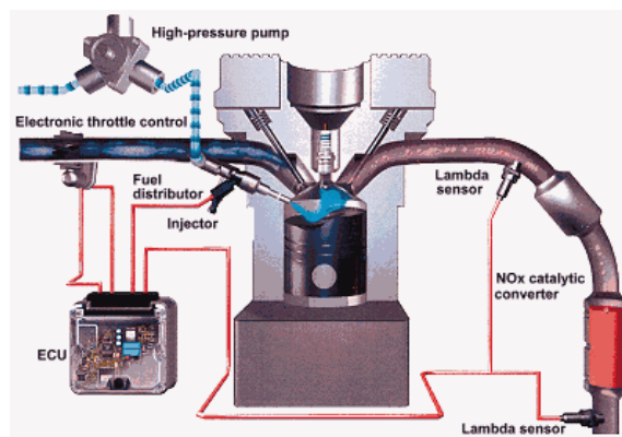
Figure 2. Schematic representation of an injection system and catalyser
