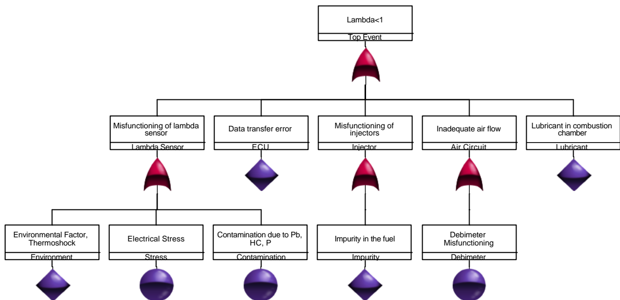
Figure 3. FTA on Top Event \lambda < 1
