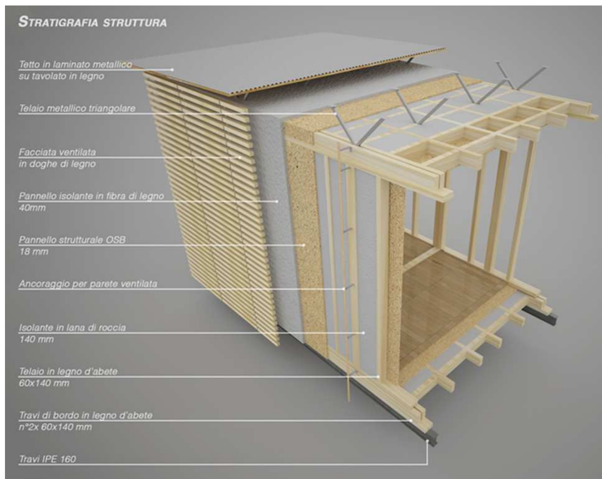
Fig. 3 The project of the innovative test cell. Rendering is made by Arch. A. Di Zenzo
