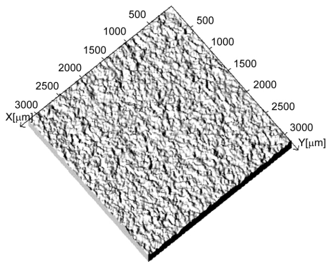
Fig. 2. Profilometric scan of the MAR M247 substrate after wet sand-blasting with 24 mesh corundum.
