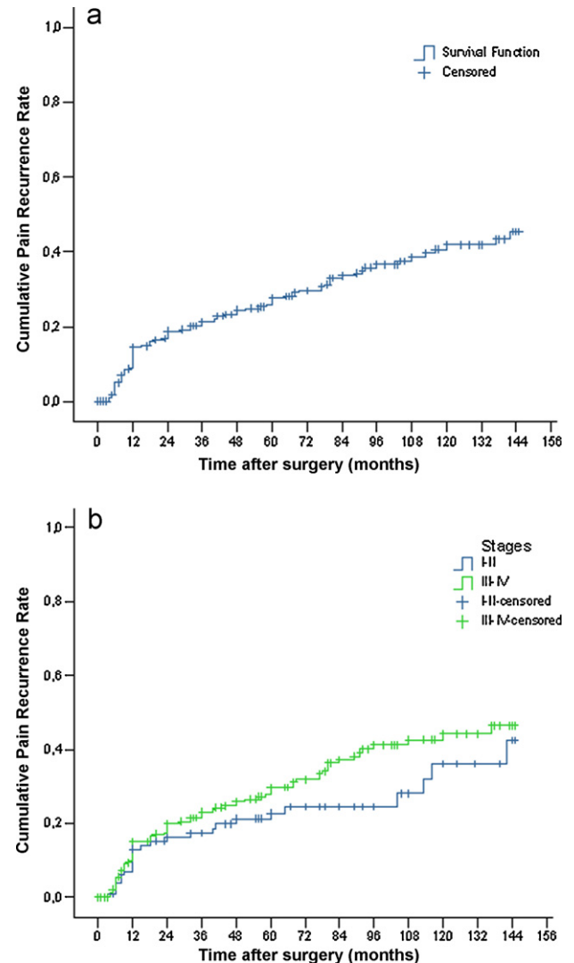
Fig. 2. Cumulative recurrence rate of pelvic pain. (A) All patients; (B) stratified according to stages (Log Rank (Mantel–Cox chi square 1832; p = 0.176 ).
