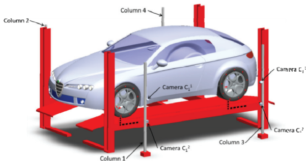
Figure 2. Acquisition system
