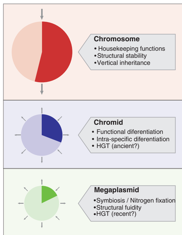
Fig. 7. —Tasks and evolutionary differences of replicons in S. meliloti .
