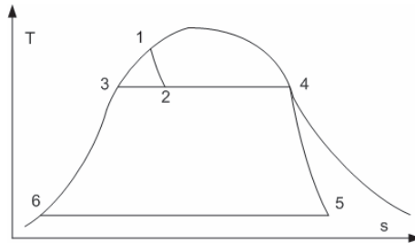
Figure 5: Single-Flash – Thermodynamic Cycle
