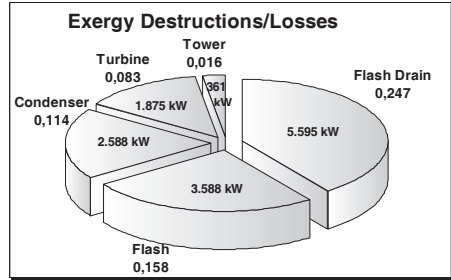
Figure 7: Single-Flash – Exergy balance. Choked well; p_c = 12,3 \text{ Pa} ; optimized at p_{sep} = 350 \text{ kPa} ; \eta_x = 0,38 .
