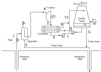
Figure 4: Single-Flash Power Plant Layout
