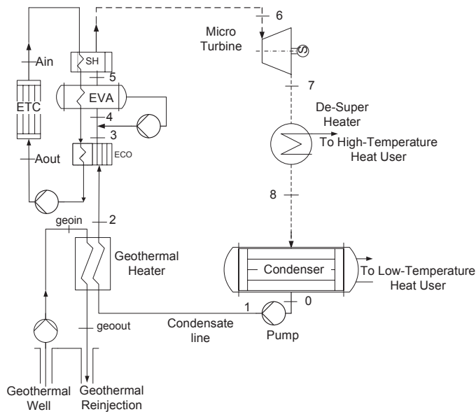
Figure 27: Integration between geothermal and solar – small CHP system
