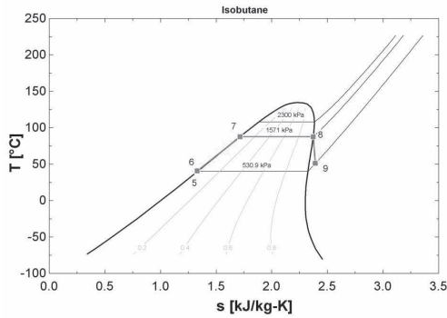
Figure 16: Example of power cycle for isobutane
