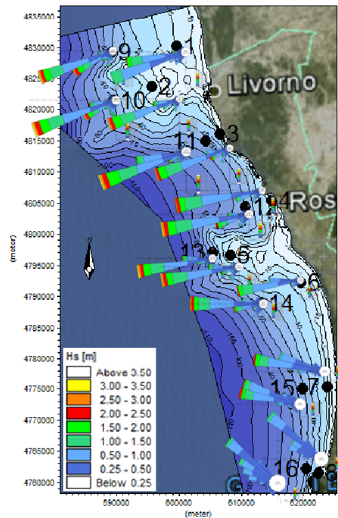
Figure 11. Central Tuscany: location and wave roses of the extracted points
