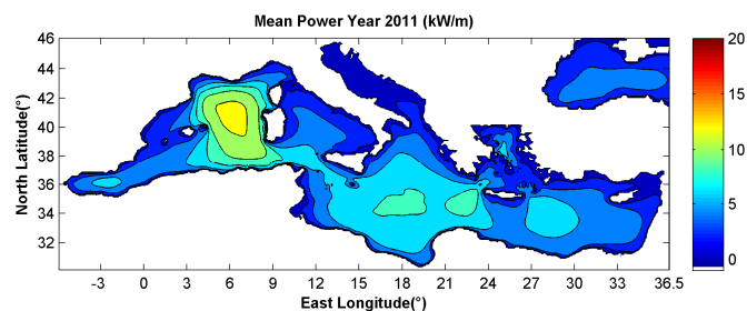
Figure 3. Spatial distribution of the Yearly Mean Power computed by using the data of the Year 2011 [kW/m]
