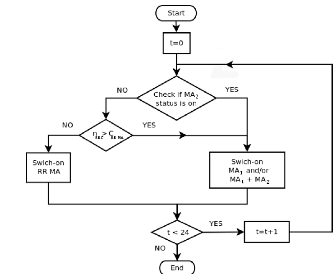
Fig. 6. Solution 2 Algorithm Flow Chart
