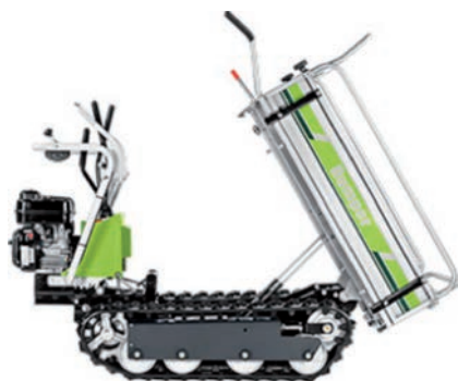
Figure 1. Grillo – mini crawler dumper- 406. The compact size (161×71×110 mm) permit to work in narrow space. The driving position is on the ground, it is provided with the automatic parking brake. Manual tipping.
