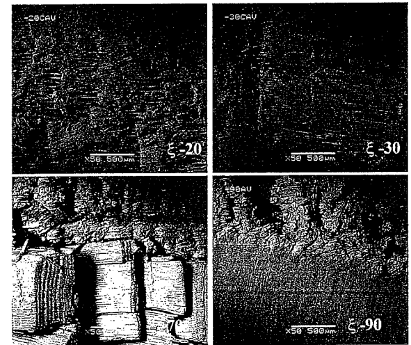
Figure 8 Douglas fir processed by down-milling, against the grain
