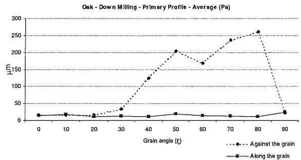
Figure 18 Pa values of oak processed by down-milling technique
