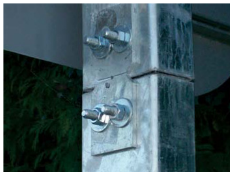
Figure 37: Breakaway/spliced pole ( left ) and slip base ( right ) [57]
