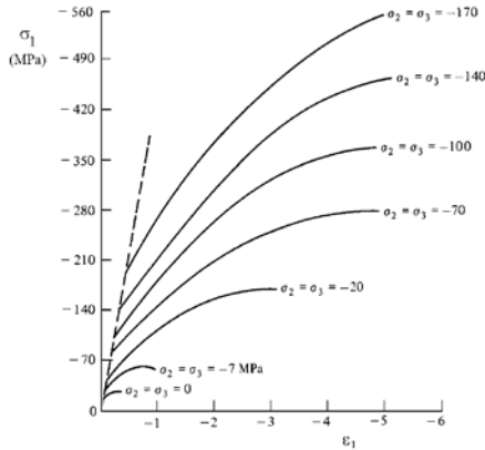
Figure 2.12 - Strength of concrete under tri-axial stress state (Chen [18])
