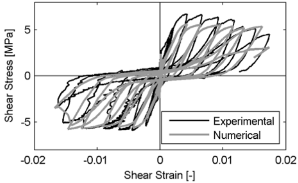
Figure 4.21 - Comparison numerical-experimental of shear stress-shear strain responses of panel CD3
