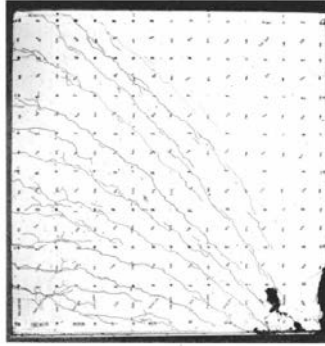
Figure 4.42 - Picture of specimen S4 at failure [12]
