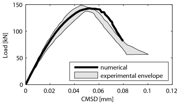
Figure 3.29 - Load-CMSD curve and comparison with experimental envelope
