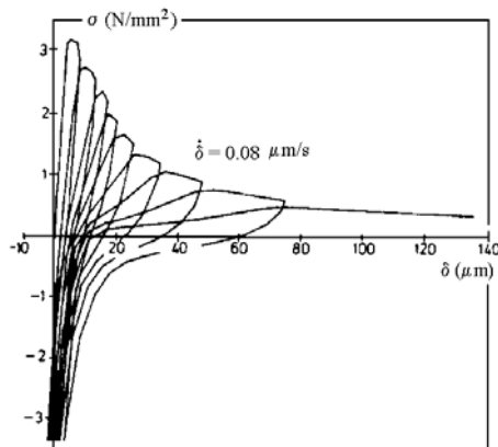
Figure 2.13 - Stiffness recovery (Yankelevsky and Reinhardt [19])
