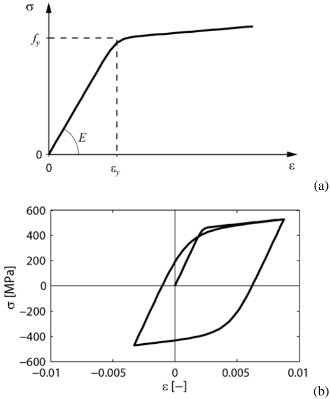
Figure 4.6 - Giuffrè-Menegotto-Pinto Law Hysteretic behavior [3]
