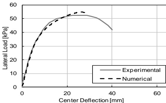
Figure 4.50 – Load-center deflection curves for numerical and experimental results
