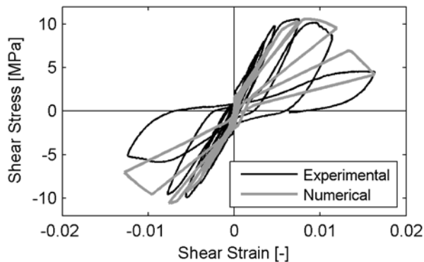
Figure 4.17 - Comparison numerical-experimental of shear stress-shear strain responses of panel CA4
