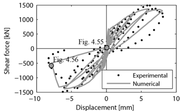
Figure 4.54 - Load-displacement curve for box-shaped shear wall and comparison with experimental data
