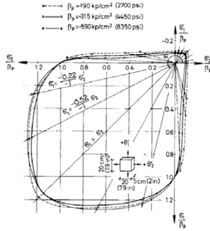
Figure 2.11 - Biaxial strength envelope (Kupfer et al. [17])
