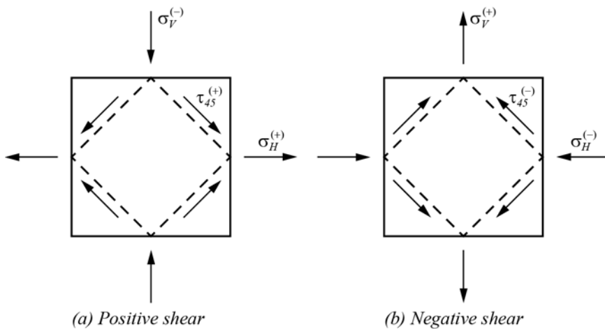
Figure 4.11 - Elements under pure shear
