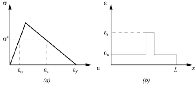
Figure 2.24 - (a) strain softening vs. elastic unloading; (b) possible strain profile along bar
