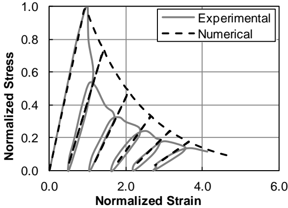
Figure 3.23 - Comparison between numerical and experimental response of a concrete specimen subjected to uniaxial cyclic tensile load
