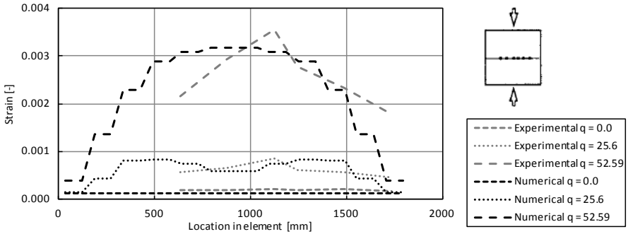
Figure 4.51 - Strains along bottom transverse bar at center of specimen and comparison with experimental data
