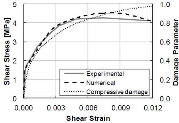
Figure 4.30 - Shear stress-shear strain curve for specimen PV20
