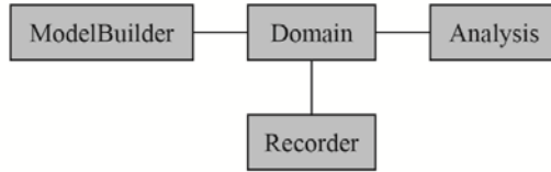
Figure 4.2 - Main abstractions of framework OpenSEES [1]
