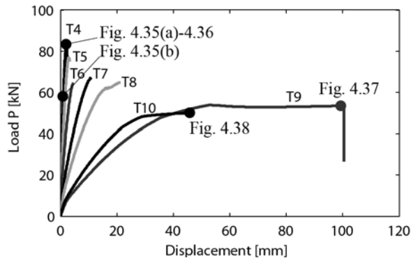
Figure 4.34 - Load-displacement curves for all beams
