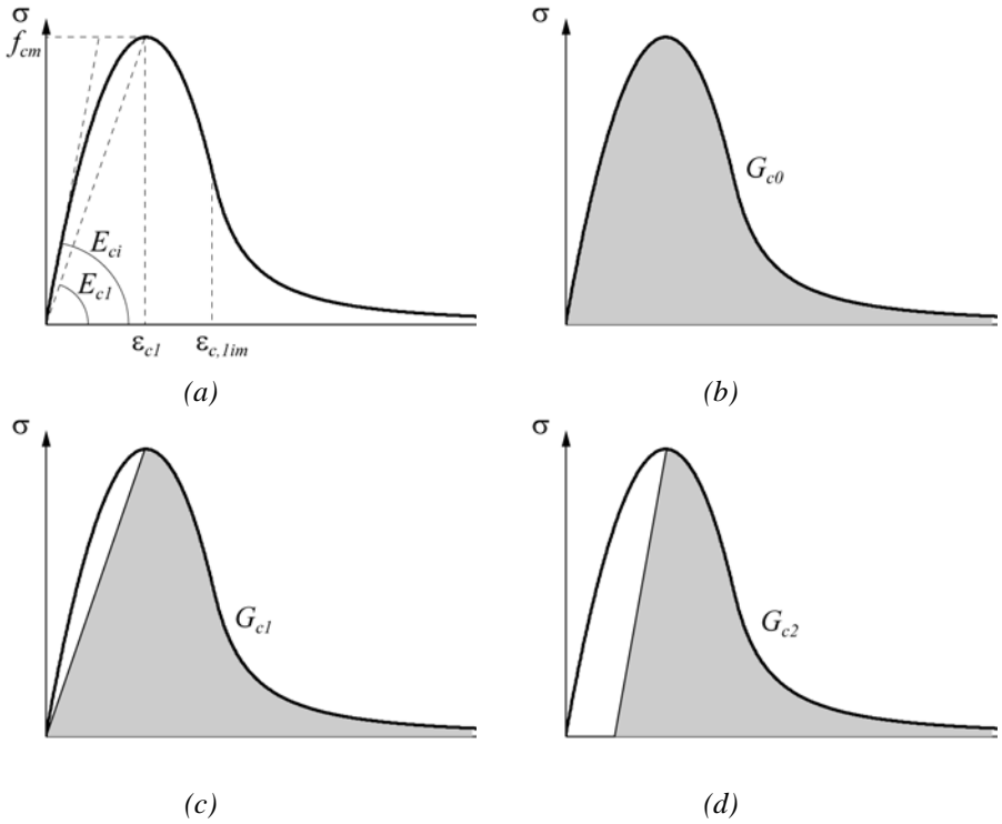
Figure 3.13 - (a) Stress-strain relation according to Model Code 1990 [21]; Crushing energy under: (b) hypothesis 0; (c) hypothesis ; (d) hypothesis 2
