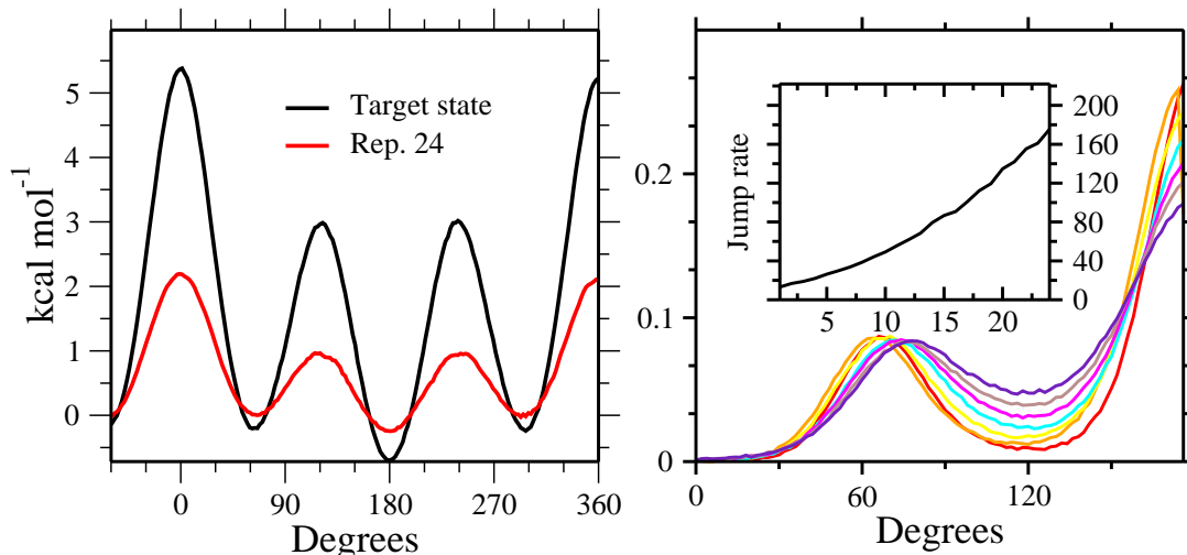
Figure 1: Left: torsional energy round the internal aliphatic C-C bond (Jämbeck type a3, see Ref. [11]); black trait, target replica; red trait, hottest replica. Right: probability distributions of the dihedral angle averaged on all aliphatic torsion angles in a non exchanging 1 ns GE simulation. Color coded scheme for distributions: from red (target state) to violet (hottest torsional state). In the inset, the jump rate per ns is reported as a function of the scaled state.
