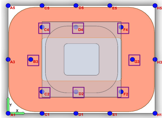
FIGURE 9. Evaluated positions of the beverage can.
