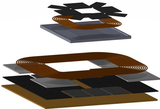
FIGURE 7. Ferromagnetic material and shielding disposition in the coils.
