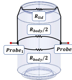
(c) Resistive model of the body.
