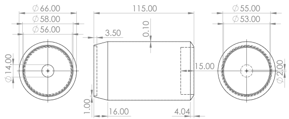
FIGURE 5. Dimensions and parts of the modelled can.
