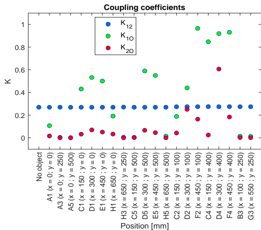
FIGURE 10. Coupling coefficients of the system for different positions of the can.
