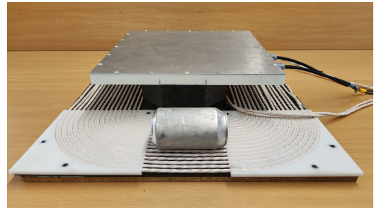
FIGURE 8. Coils with the can in the prototype.
