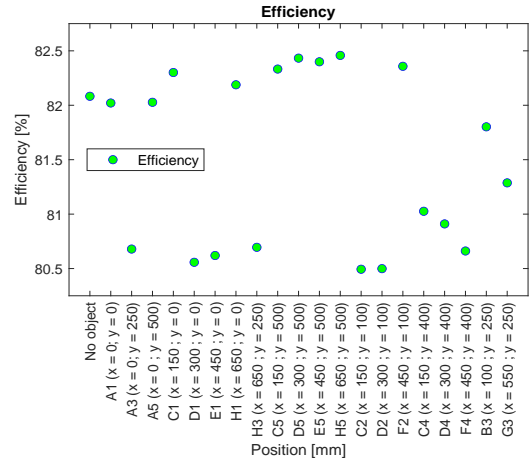
FIGURE 11. Efficiency of the system depending on the position of the can.
