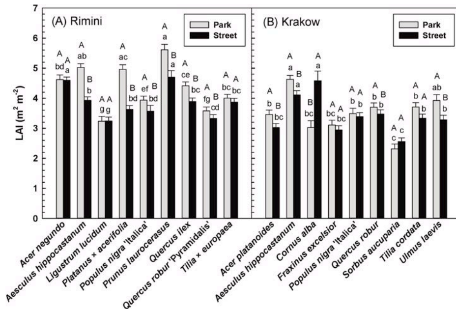
Fig. 1. Average ( \pm standard deviation) true Leaf Area Index (LAI, \text{m}^2 \text{m}^{-2} ) of park and street trees of the selected species growing in Rimini (A) and Krakow (B). For each city, different uppercase letters indicate significant differences between park and street trees within each species at P < 0.01 . Different small letters indicate significant differences among species, within each stratum, at P < 0.01 .
