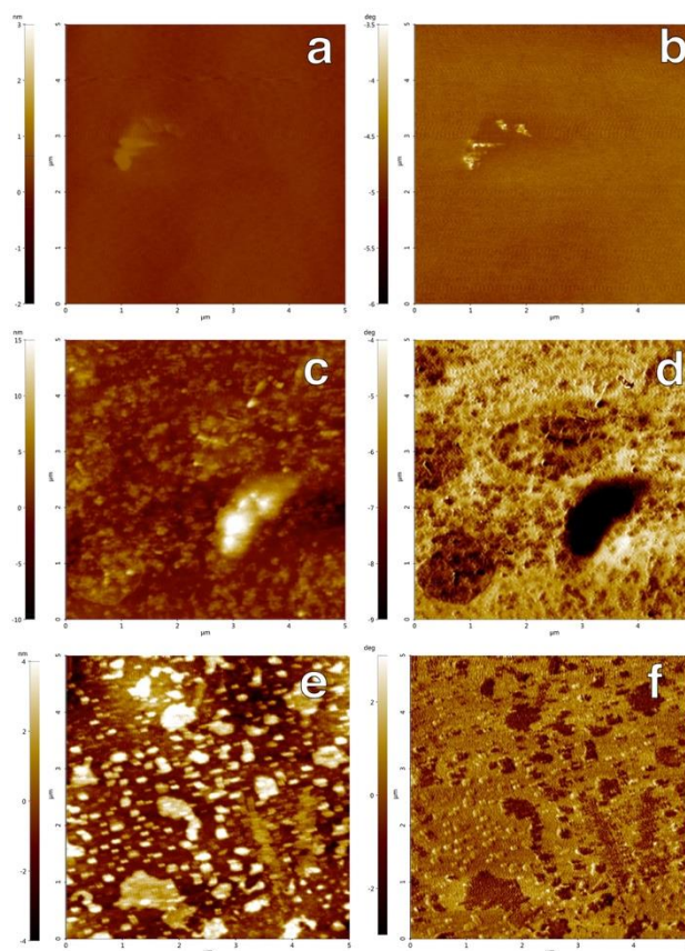
Figure 8. AFM topography and phase images of Pul (a and b, respectively), Pul-Ma (c and d, respectively) and Pul-MaUV (e and f, respectively).
