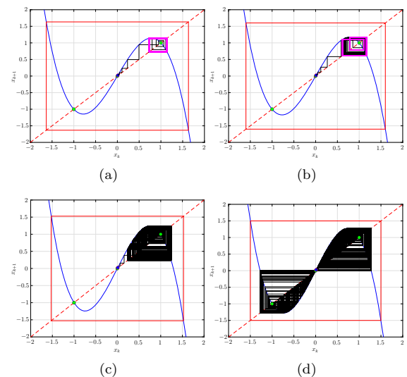
Fig. 8 Forward iterates of map (12) for different values of h . a 2-cycle for h = 1.2 ; b 4-cycle for h = 1.28 ; c single-scroll attractor encircling the fixed point 1 for h = 1.5 and d double-scroll attractor encircling the fixed points 1 and -1 for h = 1.6 . (Color figure online)
