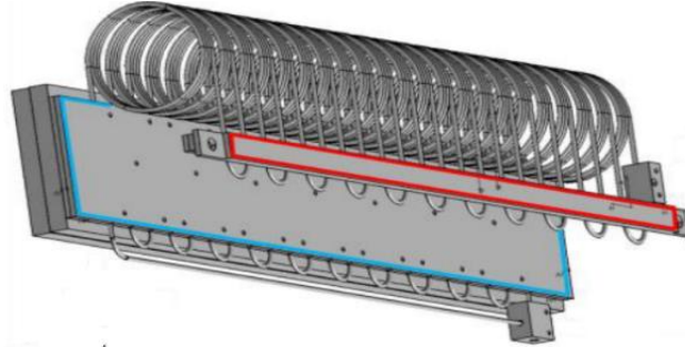
Figure 2 Deployable pulsating heat pipe (folded configuration). The heater is in red, the cold plate is in blue.
