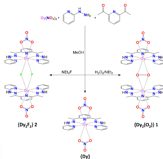
Scheme 1. Synthetic strategy used to obtain \{\text{Dy}_2(\text{O}_2)\} ( 1 ), \{\text{Dy}_2\text{F}_2\} ( 2 ) and \{\text{Dy}\} ( 3 ).
