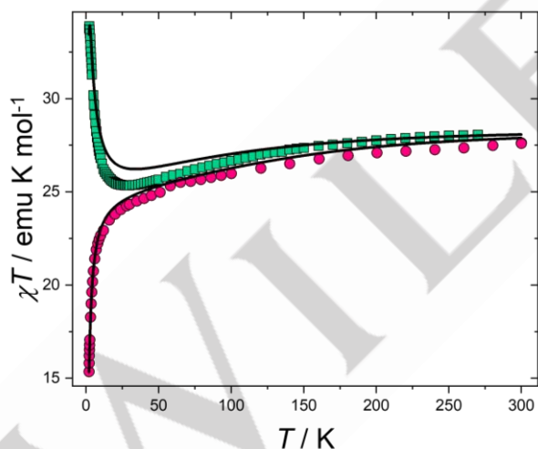
Figure 3. \chi T vs T plots for \{Dy_2F_2\} ( 1b green squares) and \{Dy_2(O_2)\} ( 2b pink circles). The black lines are the best fits (see text).
