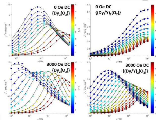
Figure 5. Out-of-phase signals for \{\text{Dy}_2(\text{O}_2)\} (left) and \{(\text{Dy}/\text{Y})_2(\text{O}_2)\} (right) in 0 dc field (top) and under 3000 Oe dc field (bottom).
