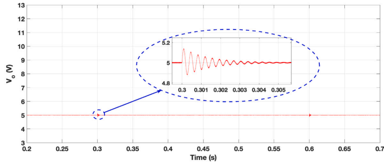
(b) Output voltage V_o
