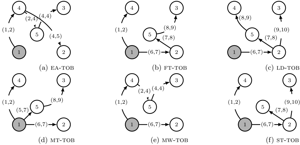
Figure 2: Example of D-TOBs of the temporal graph in Figure (1) for different distances. The grey vertex is the root of the TOB.
