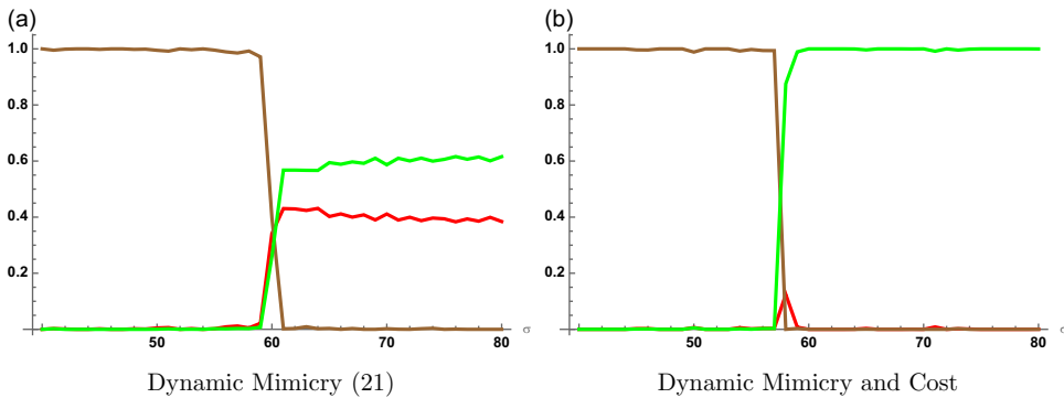
Figure 6. Population frequencies based on different payoff premia using the same parameter values as before.
