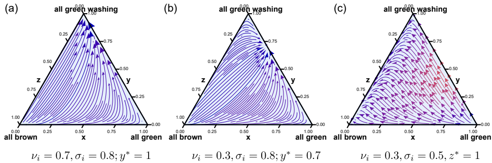
Figure 2. \beta = 1, c_i = 0.6, \mu_i = 0.4, \rho_i = 0.1, \phi_i = 100 .
