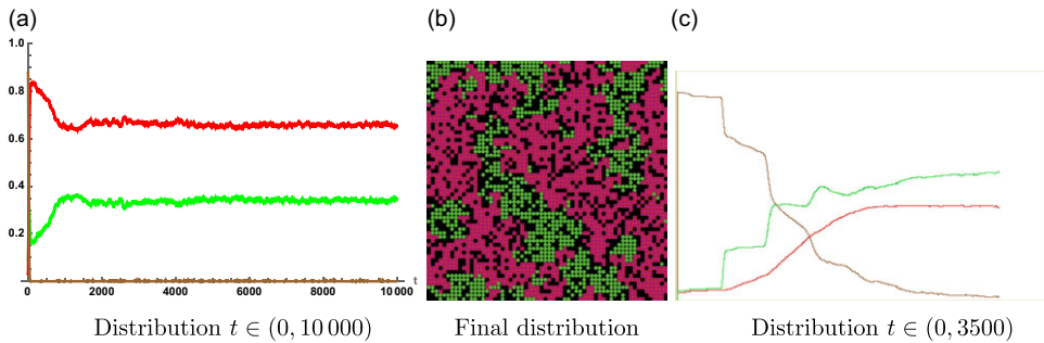
Figure 4. Strategy distribution for \sigma = 75 and \nu = 0.50 .
