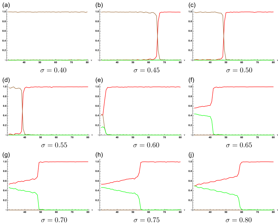
Figure 3. Equilibrium distributions for different profit premia and effectiveness of mimicry v \in [30, 80; 1] . initialization with \varphi = 100, z(0) = 0.93, x(0) = 0.04, y(0) = 0.03, c = 0.60, \mu = 0.4, \rho = 0.1, \varepsilon = 0.05 .
