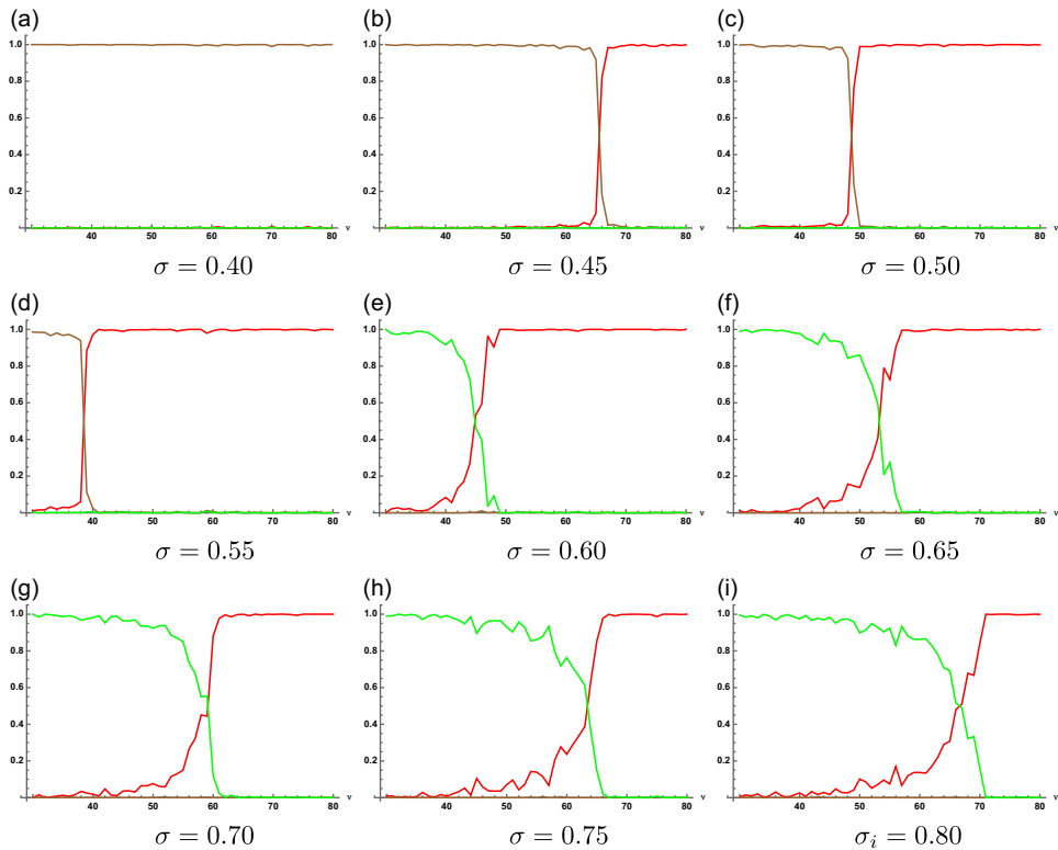
Figure 5. Dynamics for parameter values as in Figure 3 and dynamic costs according to (13).
