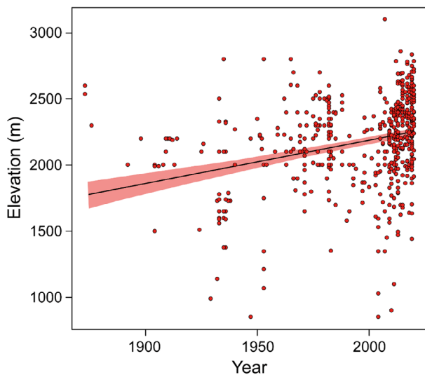
Fig 4. The relationship between year of collection and elevation for records of E. pandrose in Europe. The shaded area represents the 95% confidence interval of the regression line.
