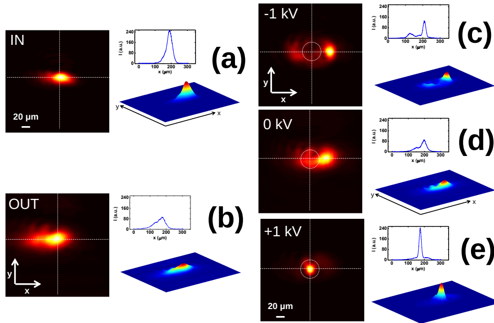
Fig. 4. IR ( \lambda = 977 nm) intensity distribution of the beam at the input facet (a) and output facet (b) (after 2.7 mm of standard linear propagation) of the crystal. Electro-driven guiding of the IR beam in a double-funnel waveguide previously written through a visible-light laser beam ( \lambda = 532 nm): intensity distribution at the output facet of the crystal for an applied voltage of -1 kV (c) (note the antiguiding central region and the guiding lateral lobes), 0 V (d) and +1 kV (e) (with the central guiding region fully activated). The central circle in (c), (d), (e) indicates the region, selected by the iris, which is imaged in the plane of the VCSEL.
