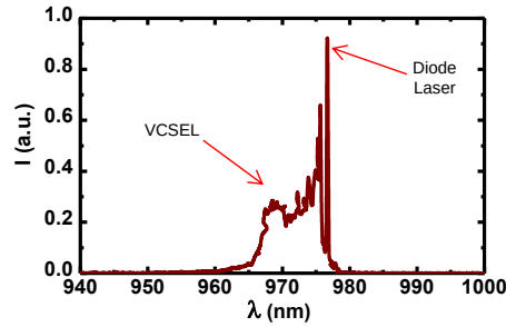
Fig. 6. Spectrum of VCSEL emission (below threshold, Fig. 3(e)) with superimposed spectrum of injected beams ( \text{FWHM} \simeq 0.43 nm) from the diode laser (LD) in experimental conditions.
